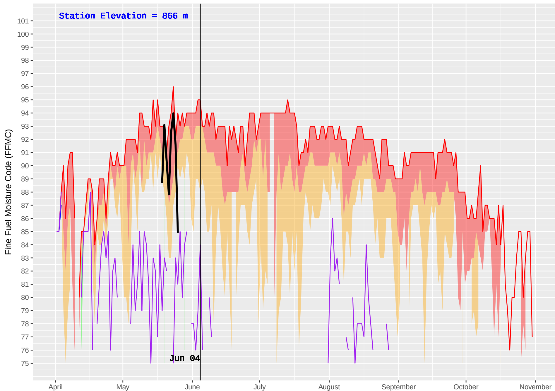
CATFISH (199) : Historical (1986–2016) and Current (2018) Noon Fine Fuel Moisture Code (FFMC)
