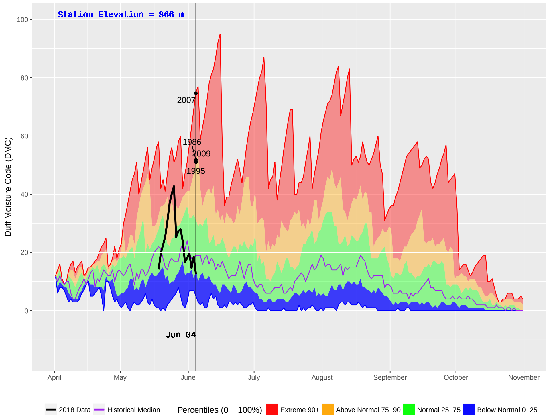
CATFISH (199) : Historical (1986–2016) and Current (2018) Noon Duff Moisture Code (DMC)
