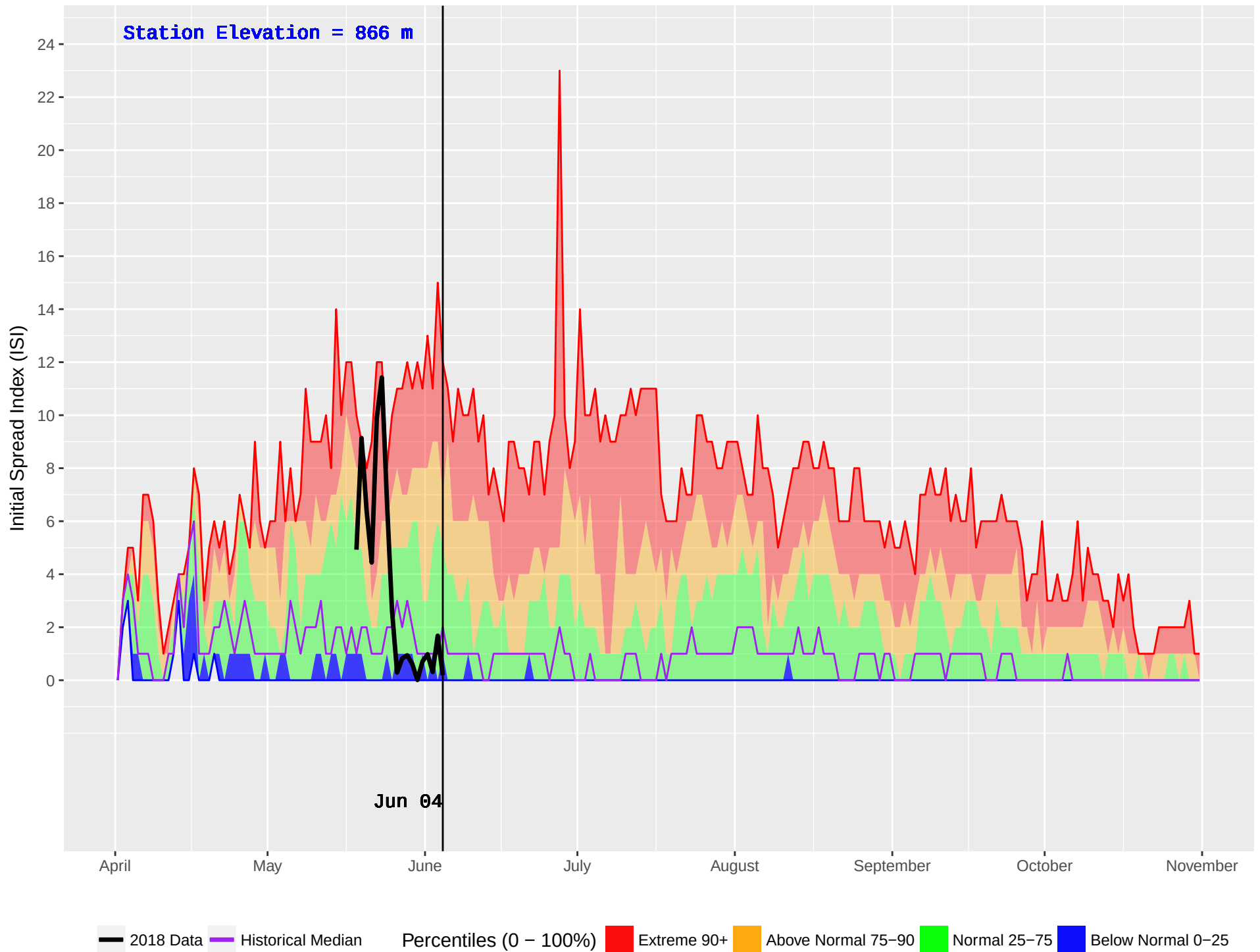
CATFISH (199) : Historical (1986–2016) and Current (2018) Noon Initial Spread Index (ISI)
